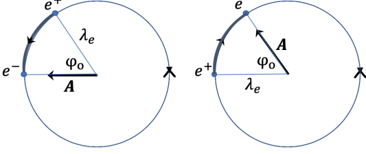
FIG. 4: Photon structure: A photon is composed of an electron-positron pair circulating at the speed of light with a fixed angular separation \varphi_0 , where 0 \leq \varphi_0 \leq \pm\pi designates left and right circular polarizations.
