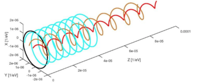
FIG. 6: Picture the photon as a moving ring with angular momentum \hbar that generates an electromagnetic wave with amplitude normalized to its energy. (Figure from [51] with a different but related interpretation)
