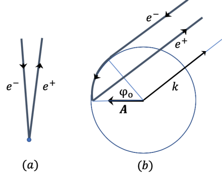
FIG. 5: Photon propagation: (a) Feynman diagram for pair creation (b) Photon propagation is centered along a lightlike path with tangent vector k .
