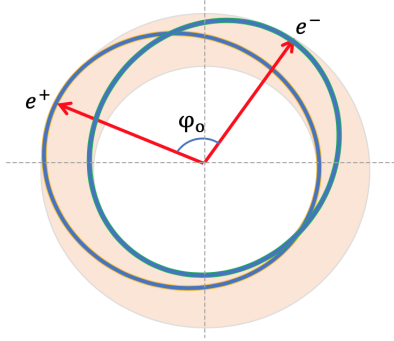
FIG. 7: The photon can be modeled as an electron-positron pair located on a toroidal ring (or energy shell) with a fixed angular separation \varphi_0 designating its polarization.
