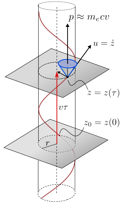
FIG. 2: In the Zitter Particle Model the electron path is an oriented lightlike helix with an opposite orientation for a positron.
