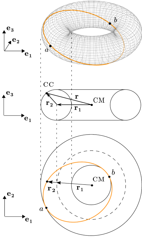
FIG. 3: In a plane rotating with angular velocity \omega_1\sigma_3 around the CM, the electron's lightlike circular orbit lies on a toroidal surface called the electron energy shell that projects to the orbital plane as an ellipse with antipodes a and b .
